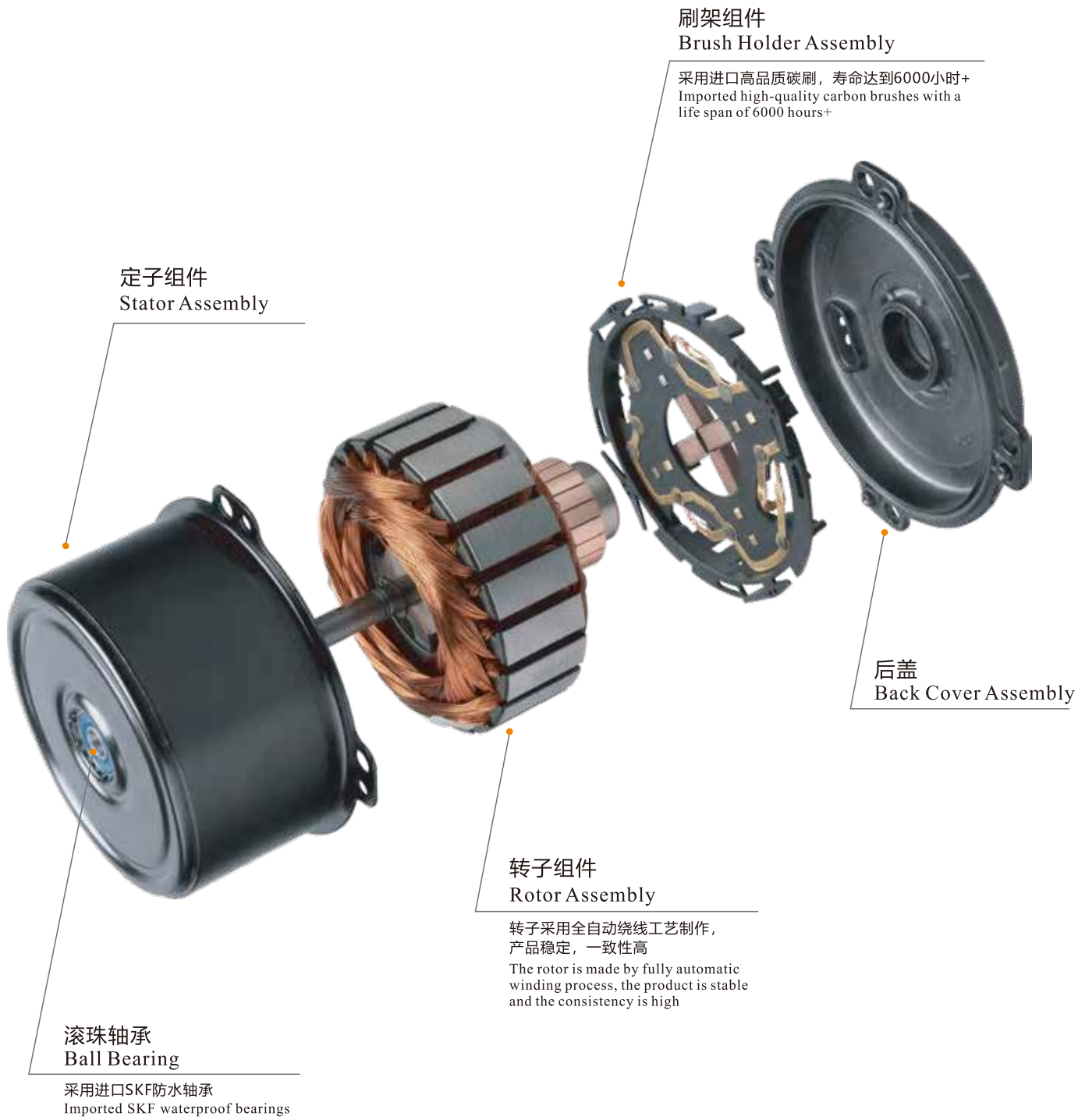
防护等级IP68冷凝电机结构图 The drawing of IP68 condenser fan motor
